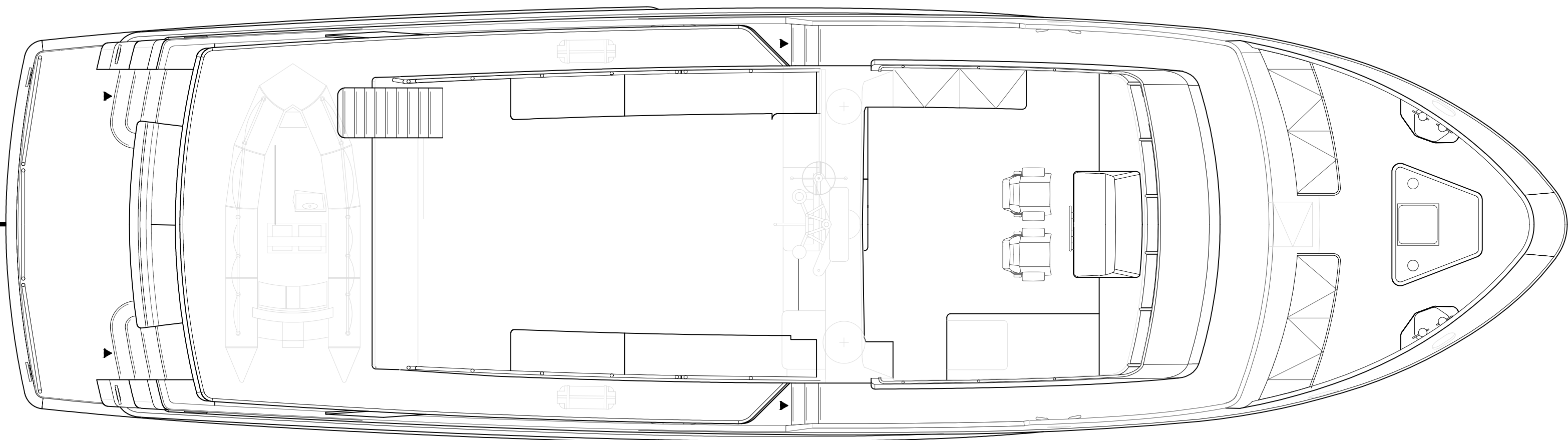
FLYING BRIDGE DECK
