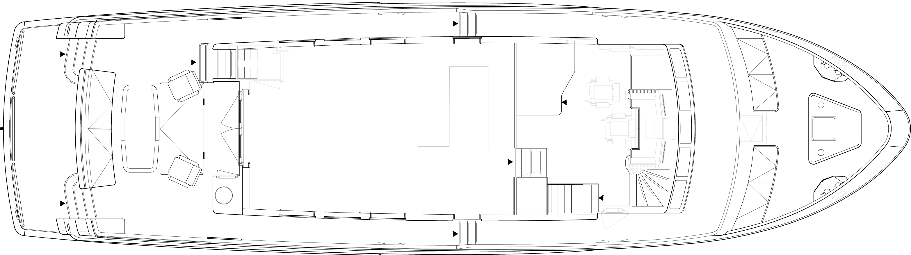
MAIN DECK
