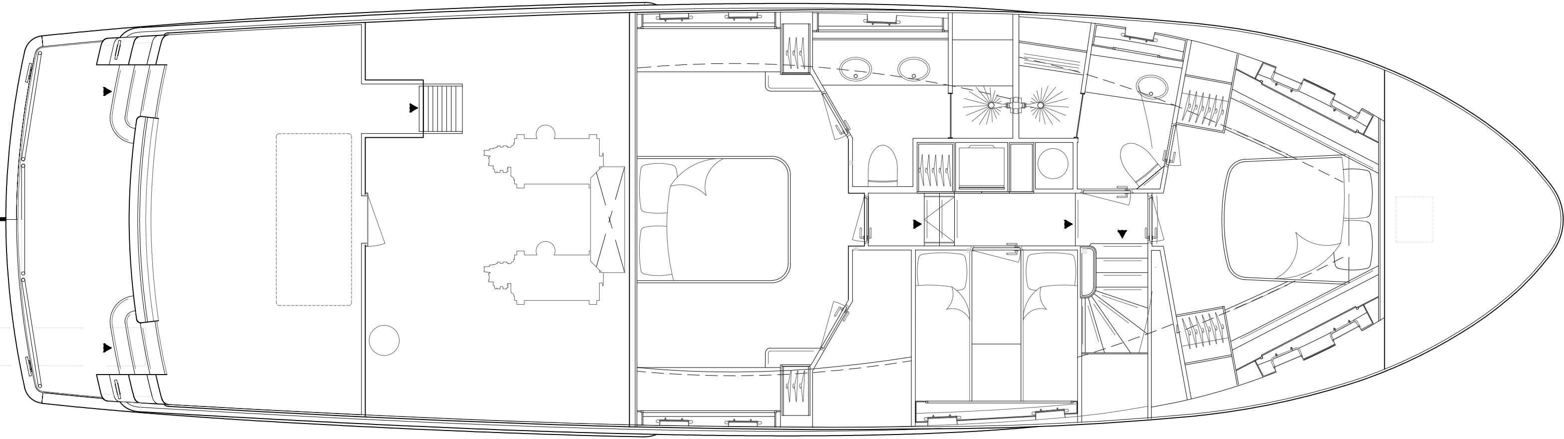
LOWER DECK
